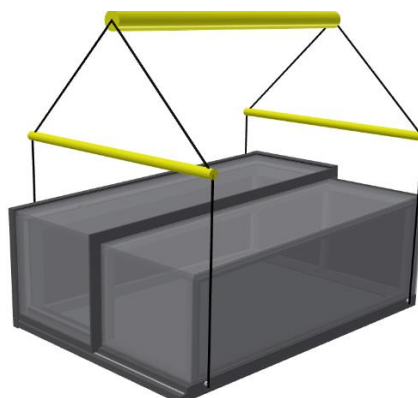
Figure 6 – Suggested lifting configuration
