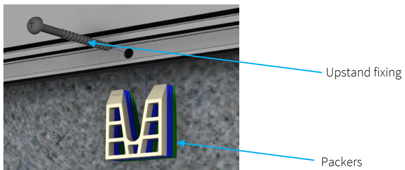
Figure 8 - Upstand fixings
