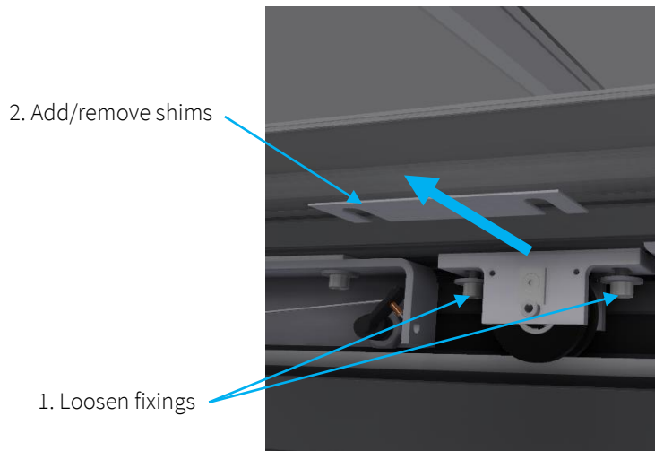
Figure 9 – Adjust door position
