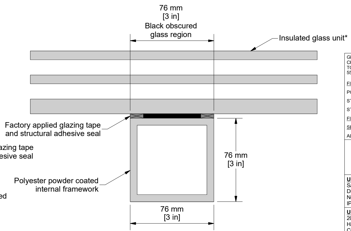
Detail K ( Scale 1 : 2 )
