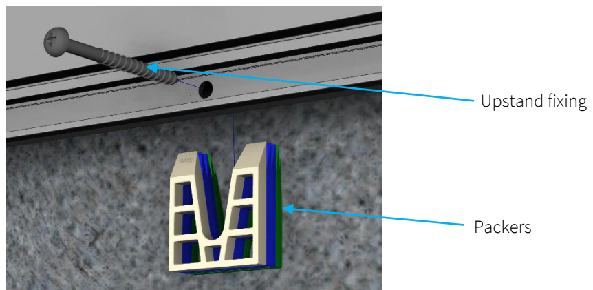
Figure 11 - Upstand fixings
