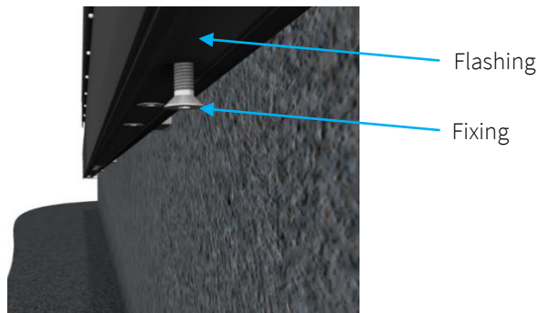
Figure 12 – Flashing fixings
