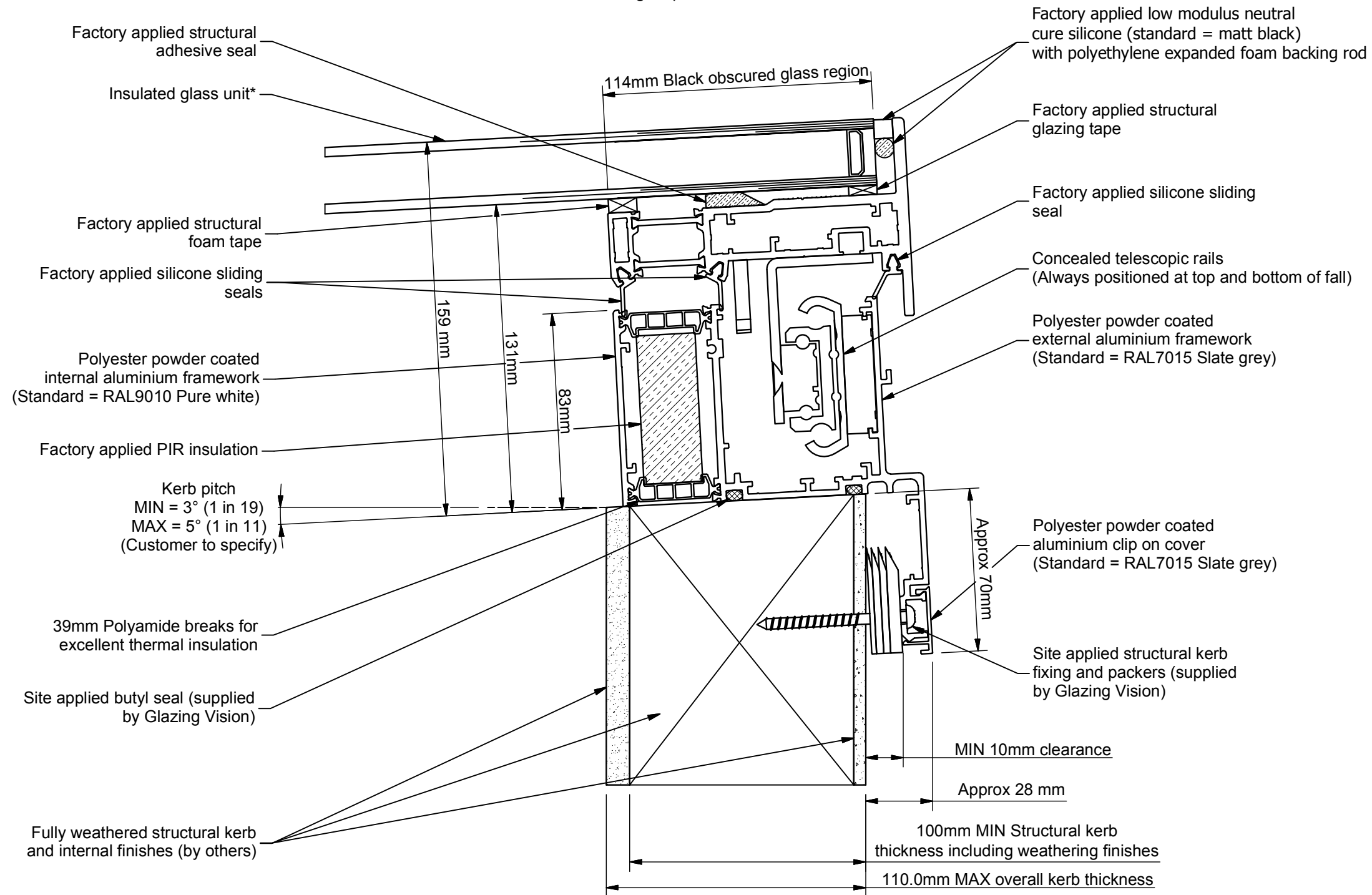
Detail C ( Scale 1:2 ) Section through top of fall
