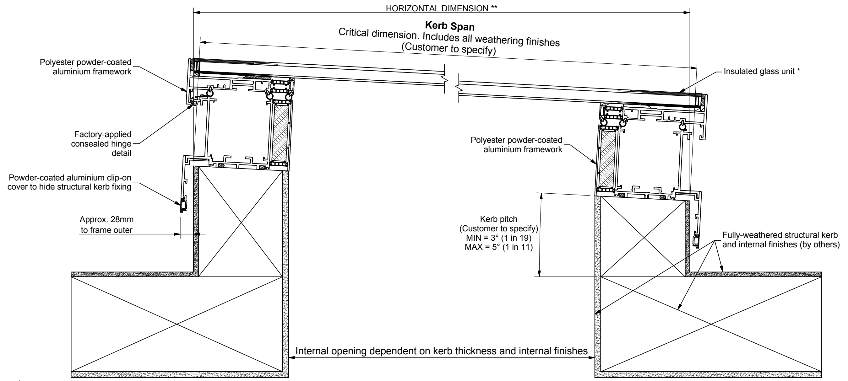
Section B-B ( Scale 1 : 5 ) (Along fall)
